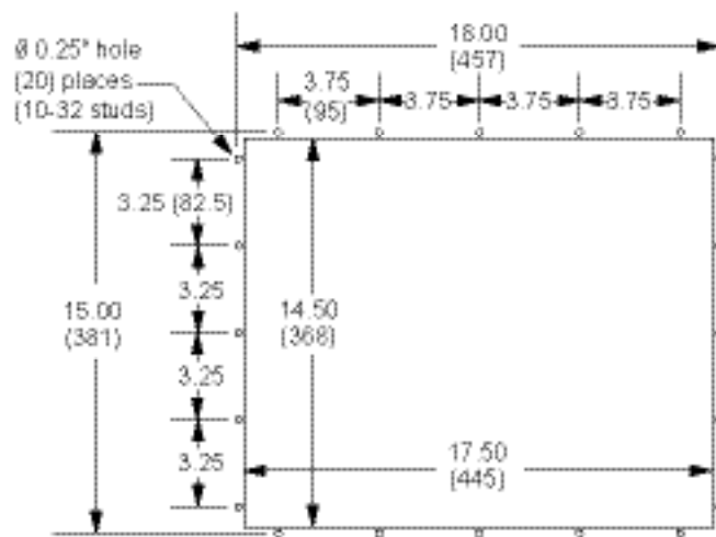
Panel Cut-Out
